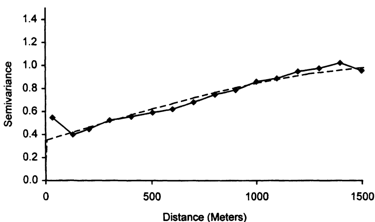
Figure 7.10 Semivariogram of normal scores of porosities computed from geophysical logs (solid line) and fitted model (dashed line) in the horizontal direction.
