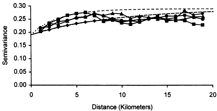
Figure 6.6 Directional semivariograms and anisotropic model of gas initial potential for the 792 Mcfpd cutoff. Directions are diamonds: north-south; filled circles: northeast-southwest; squares: east-west; and triangles: southeast-northwest. The model represented by the long dashes is for the north-south direction, the other for the east-west direction.
