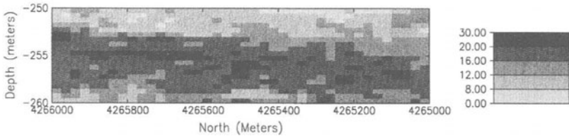
Figure 7.14 North-south cross-section of log porosities (in per cent) from sequential Gaussian simulation. Cross-section is located at 487000 m East.
