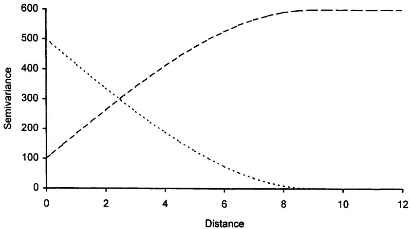
Figure 2.14 Comparison of covariance with the equivalent semivariogram.
