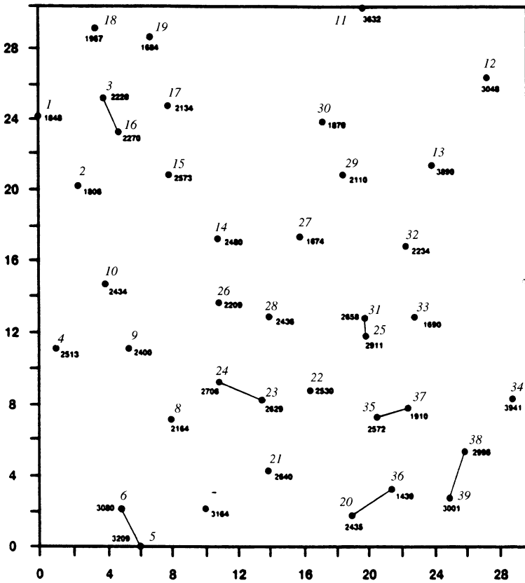
Figure 2.2 Sample location map of Paleocene clastic thicknesses taken from Gumati and Kanen (1985). Solid lines connect points separated by distances between one and three units.
