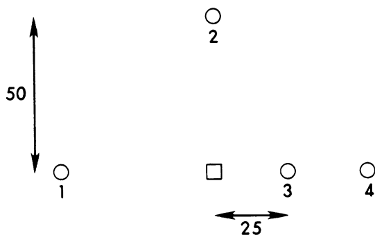
Figure 3.4 A third hypothetical configuration of control points.
