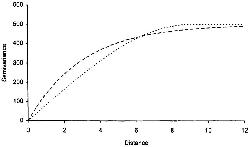
Figure 2.11 Graphical comparison of spherical (dotted line) and exponential (dashed line) models for the semivariogram.
