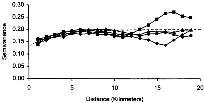
Figure 6.5 Directional semivariograms and model of gas initial potential in Barbour County for the 400 Mcfpd cutoff. Directions are diamonds: north-south; filled circles: northeast-southwest; squares: east-west; and triangles: southeast-northwest. Dashed line shows the isotropic model.
