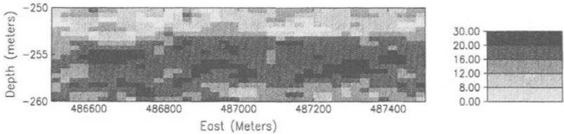
Figure 7.13 East-west cross section of log porosities (in per cent) from sequential Gaussian simulation. Cross-section is located at 4265500 m North.
