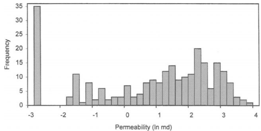
Figure 2.42 Histogram of the natural log of permeability in Granny Creek field.
