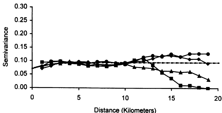
Figure 6.8 Directional semivariograms and model for gas initial potential at 2477 Mcfpd cutoff. Directions are diamonds: north-south; filled circles: northeast-southwest; squares: east-west; and triangles: southeast-northwest. Dashed line shows the isotropic model.
