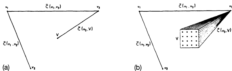
Figure 3.1 Some of the terms in the kriging equations for (a) point kriging and (b) block kriging.
