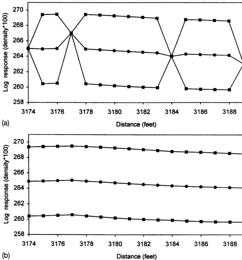
Figure 3.6 Kriged estimates (filled circles) and standard error (squares) along a transect for a semivariogram model with large nugget effect. In (a) some of the estimated locations coincide with the observed points, and therefore estimates equal observed values and estimation variance is zero; in (b) the estimated locations do not coincide with the observed points.
