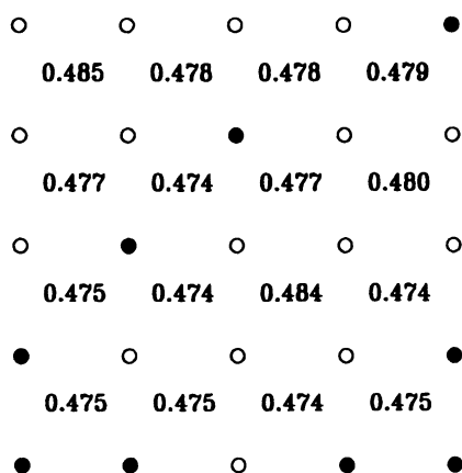
Figure 4.2 Estimation variance of the undersampled variable obtained by cokriging with a relatively large cross-covariance.
