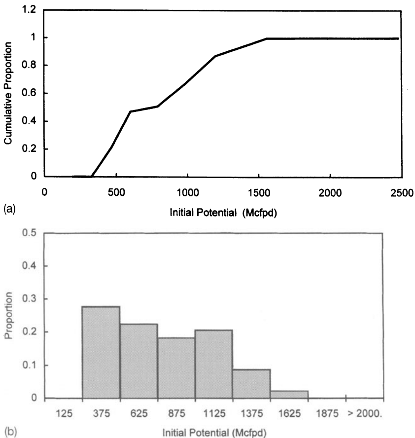
Figure 6.17 Local cumulative distribution and histogram of initial potential at location A in Fig. 6.16.
