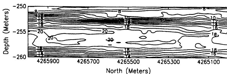
Figure 3.20 North-south cross-section through three-dimensional model of porosity in Granny Creek field at coordinate 487000 East in Fig. 3.18.
